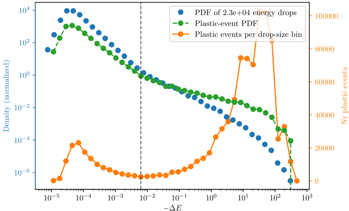
Energy-drop PDF and plasticity vs drop size
