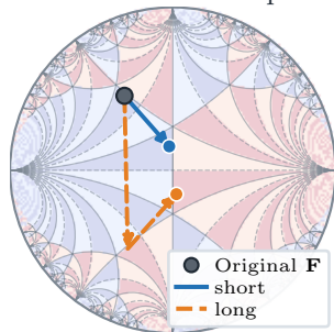
Poincaré disk: BFS paths
