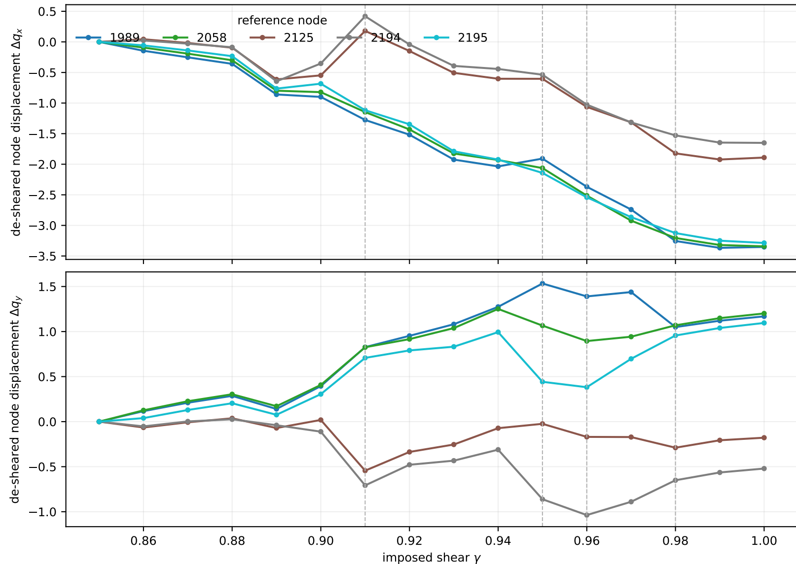
Physical nodes involved in the late element-4250 reconnections
