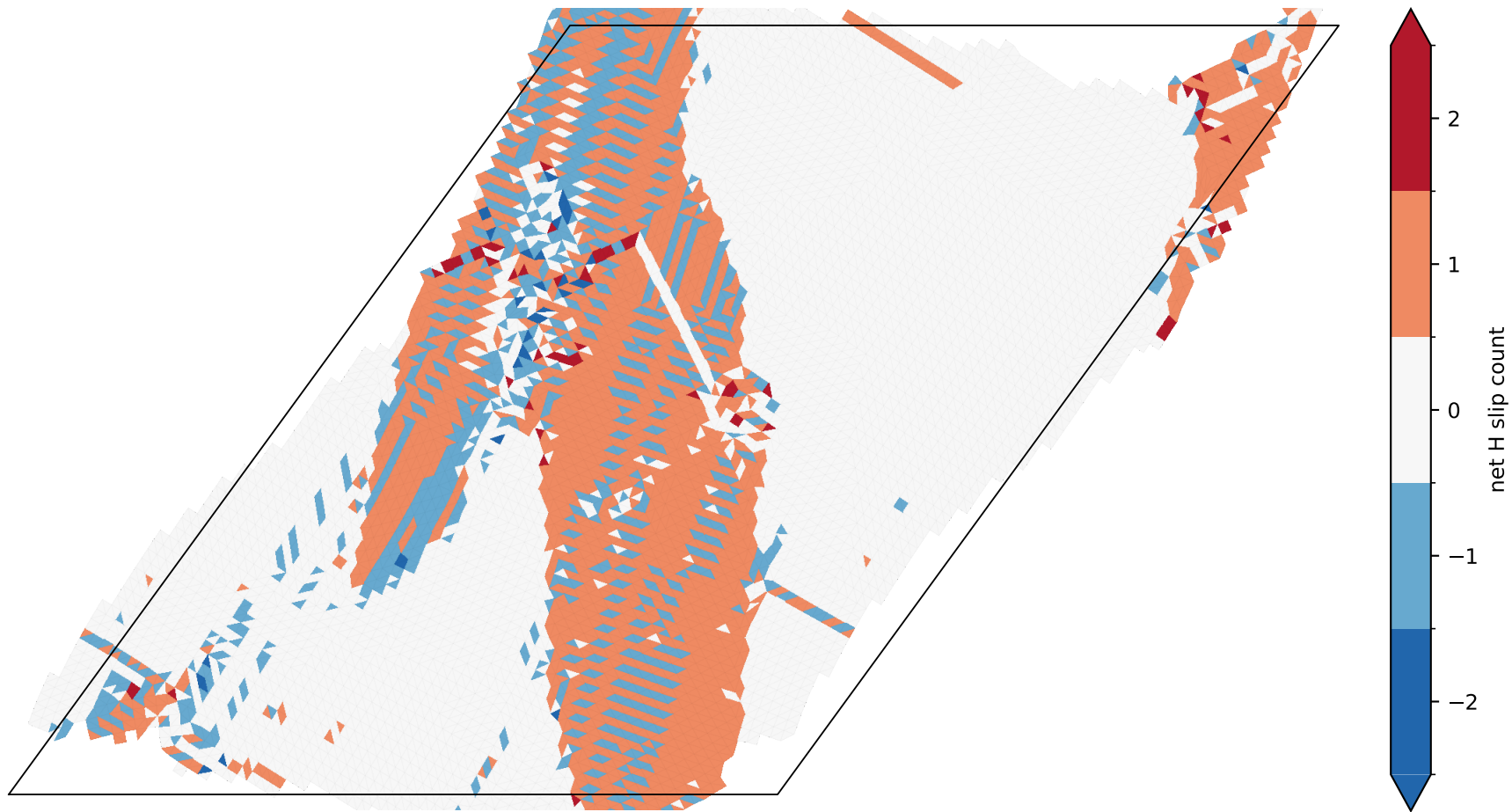
Reconstructed history T_{\text{total}} net H field at \gamma = 0.73 ; 9 values saturated
