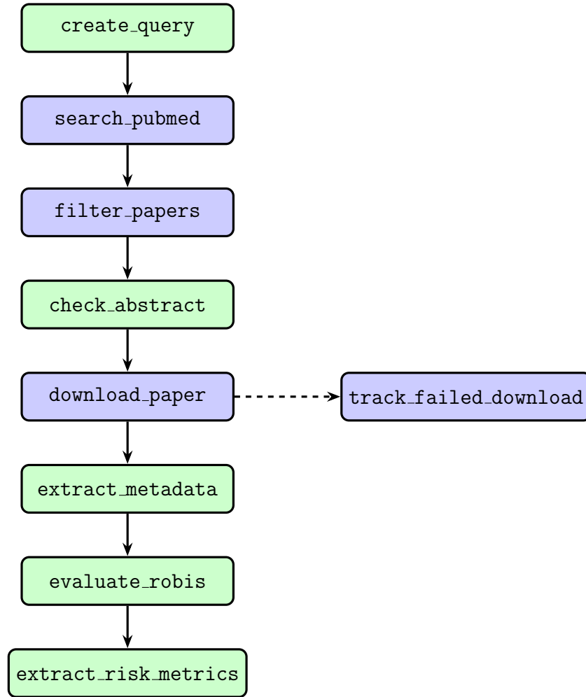
Figure 1: Agent processing nodes in sequential order. Green = AI-powered nodes, Blue = tool/logic nodes. Dashed line shows alternative path for failed downloads.
