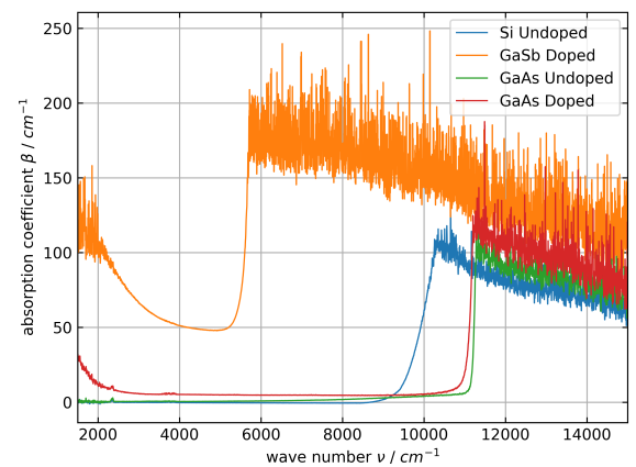
Abbildung 9: Absorption coefficient \beta of different semiconductor samples.
