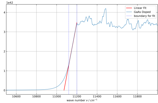
Abbildung 12: Determination of the bandgap.
