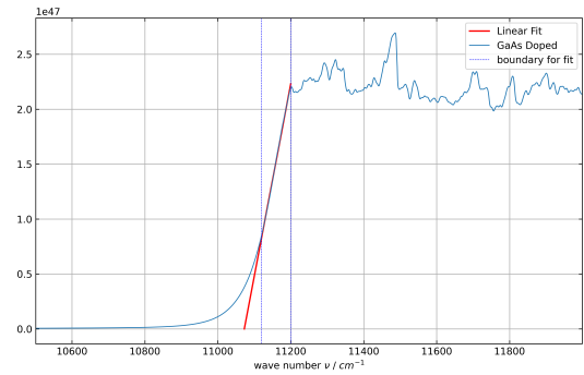
Abbildung 12: Determination of the bandgap.
