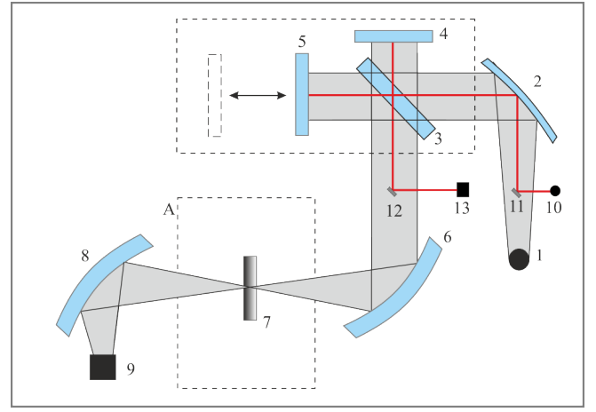
Abbildung 5: Simplified schematic illustration of the set-up used for all experiments. A short overview of the working principle is given in the text.[4]
