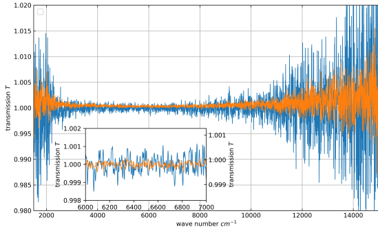
Abbildung 7: Transmission measurements for N_{\text{scan}} = 10 and N_{\text{scan}} = 100 mirror passes. The inset shows the part used for evaluation of the signal to noise ratio (see fig. 8)
