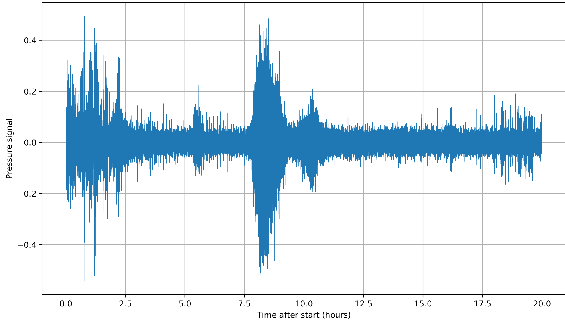
Raw pressure signal from AM.R0033_unfilt.h5
