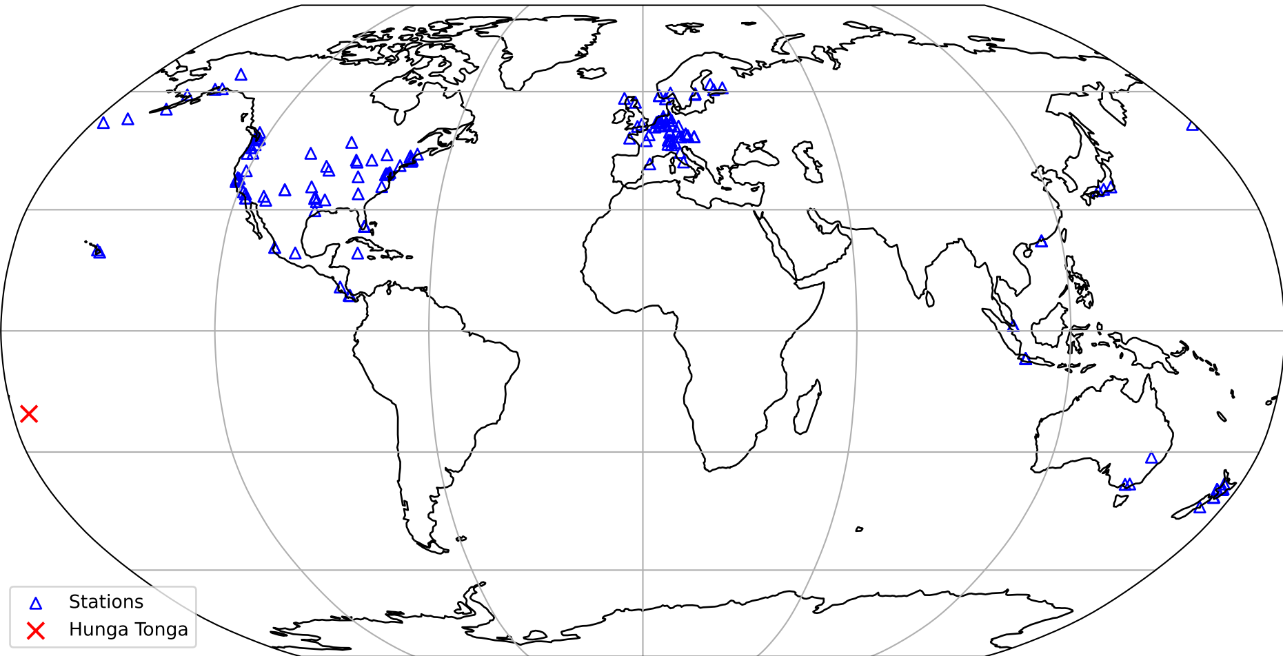
Hunga Tonga and measurement stations
