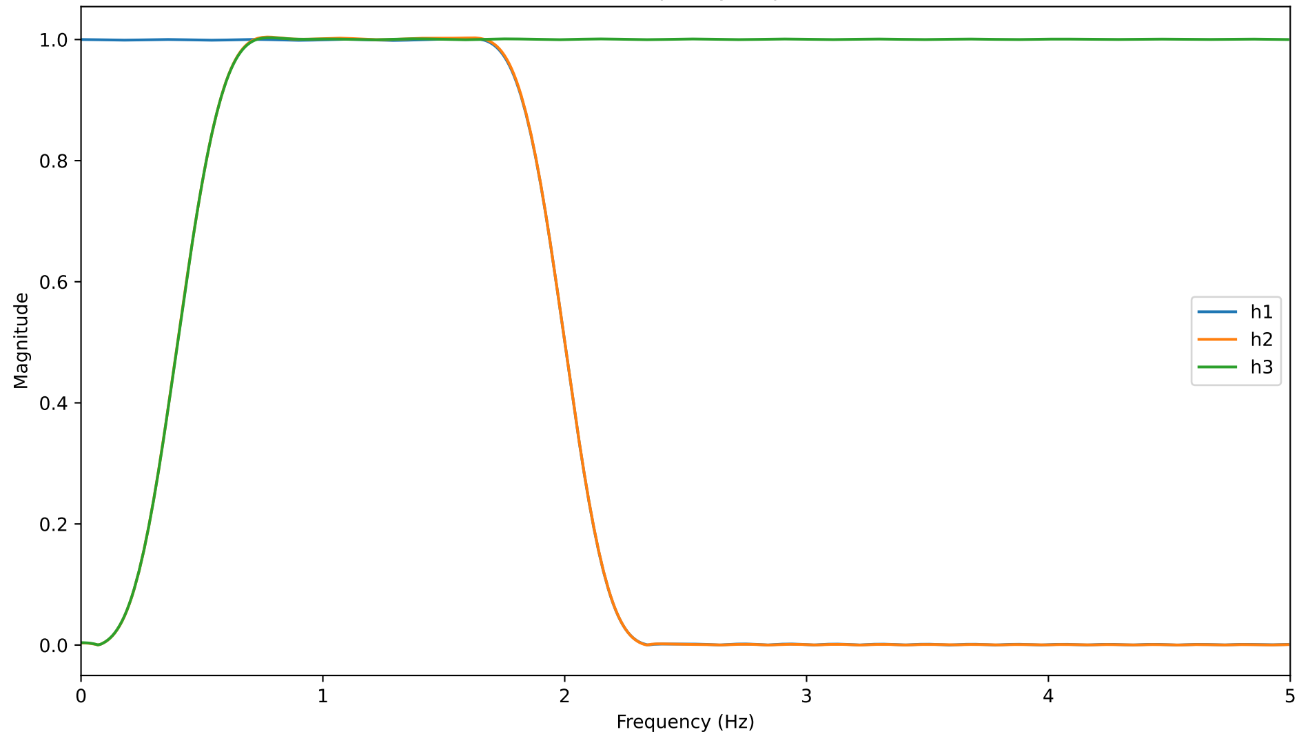
FIR filter frequency responses
