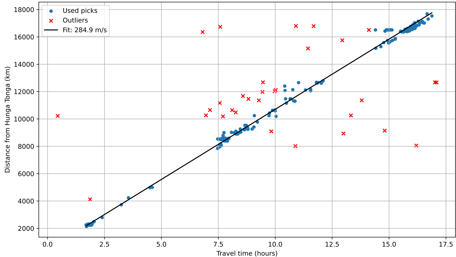
Infrasound arrival times and celerity estimate
