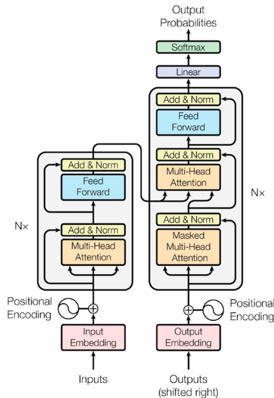
Figure 1.2: Architecture Transformer [43]
