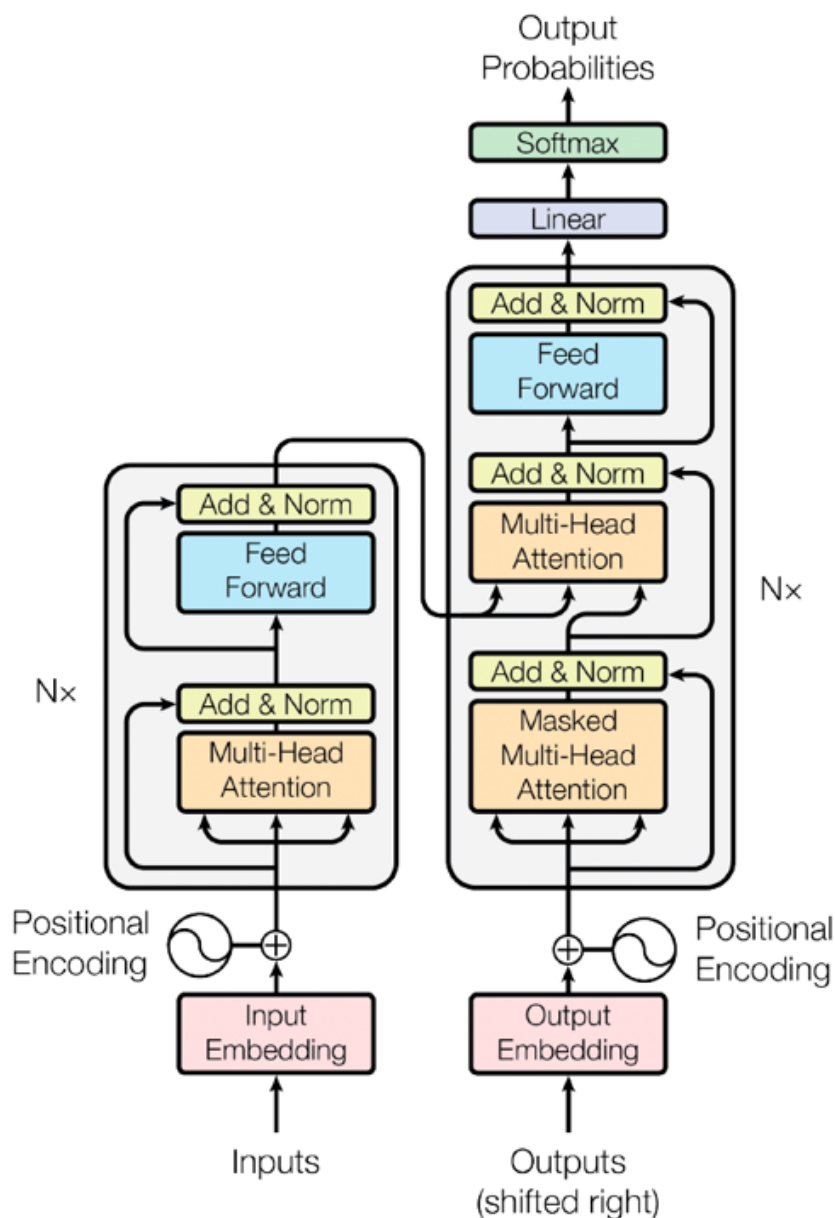
FIGURE 1.3 – Architecture Transformer [48]
