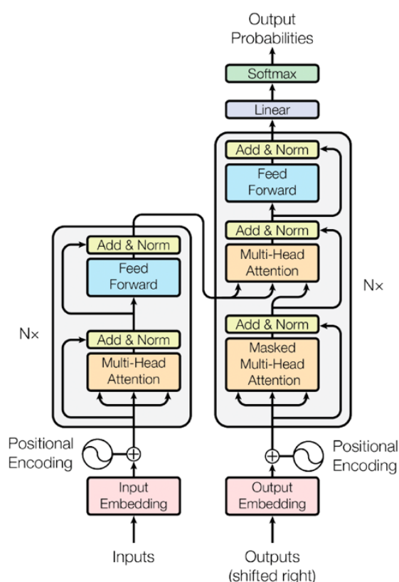
Figure 1.2: Architecture Transformer [31]
