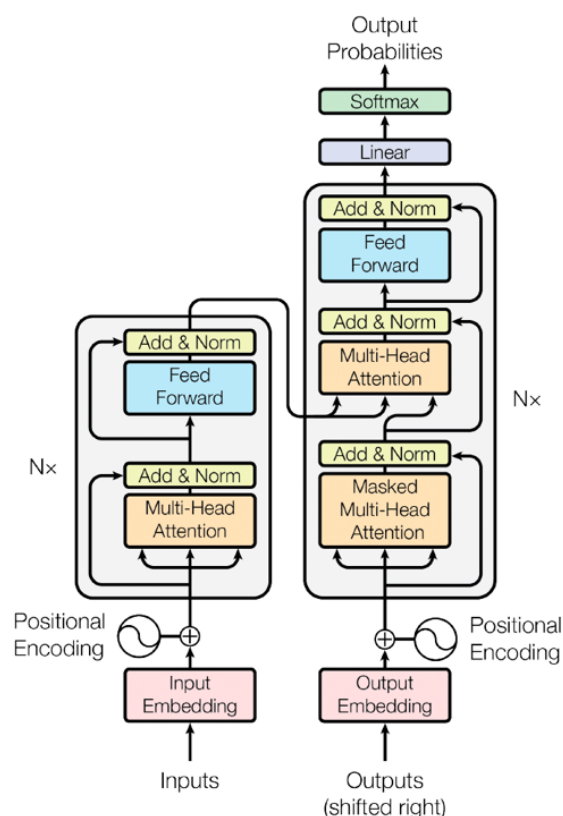
Figure 1.2: Architecture Transformer [31]
