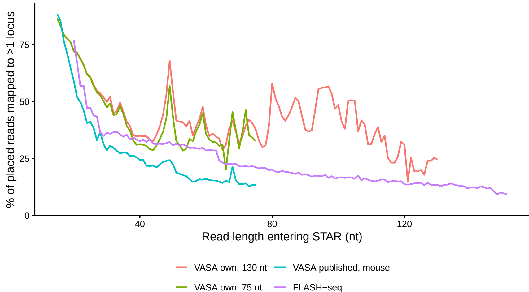
Multimapping rate against read length
