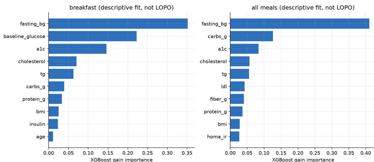
Figure 4 — Feature importance for iAUC. Descriptive fit on all available data (not LOPO); shown for interpretation, never used for model selection.
