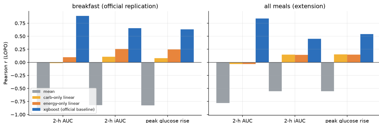
Figure 2 — Model comparison. Out-of-fold Pearson r by model, target and subset. XGBoost dominates everywhere; the linear baselines are close to zero, and the mean predictor is negative by construction. The sign is worth explaining: under LOPO the "mean" model predicts the mean of the other 44 subjects, so for a high-responding person that mean is pulled down by that person's own exclusion. The leave-one-out mean is therefore anti-correlated with the held-out subject, which is why this no-skill reference lands below zero (and below 0.5 ROC-AUC) instead of at zero. It is a reference point, not a model that has learned anything.
