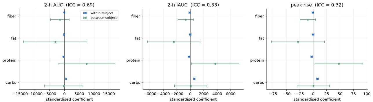
Figure 8 — Mixed model (subject random intercept). Standardised within- and between-subject coefficients with 95% intervals; each panel has its own x-scale because the targets differ by orders of magnitude.
