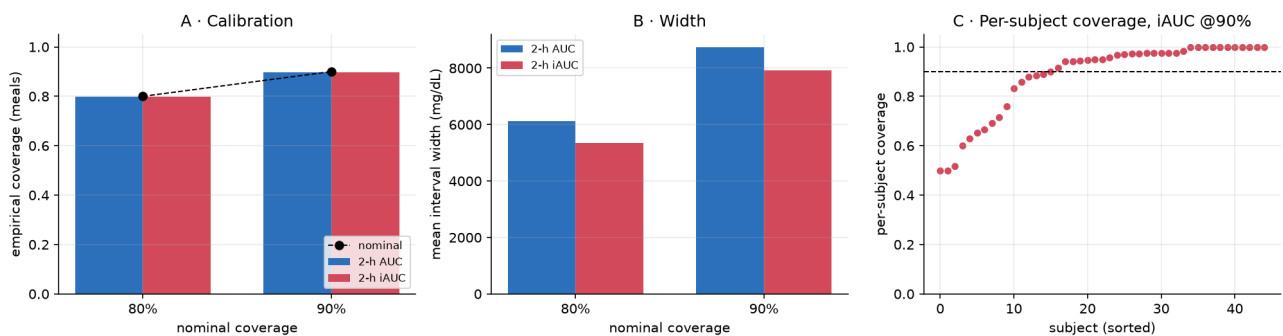
Figure 7 — Conformal intervals. A: empirical versus nominal coverage. B: interval width. C: per-subject coverage at 90% for iAUC, sorted — the tail below the dashed line is the exchangeability caveat made visible.
