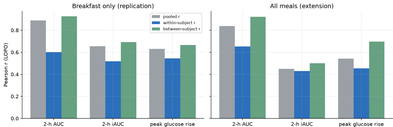
Figure 6 — Pooled skill versus its within- and between-subject parts (XGBoost, LOPO). When the between-subject bar towers over the within-subject bar, much of the pooled correlation reflects knowing who the person is.
