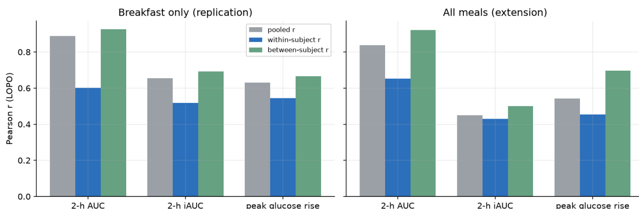
Figure 6 — Pooled skill versus its within- and between-subject parts (XGBoost, LOPO). When the between-subject bar towers over the within-subject bar, much of the pooled correlation reflects knowing who the person is.
