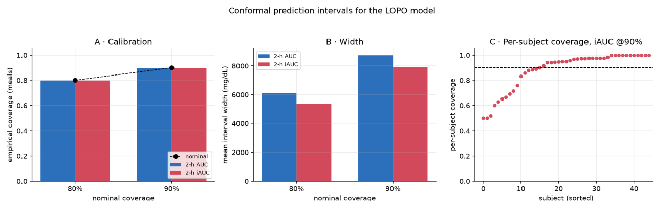
Figure 7 — Conformal intervals. A: empirical versus nominal coverage. B: interval width. C: per-subject coverage at 90% for iAUC, sorted — the tail below the dashed line is the exchangeability caveat made visible.
