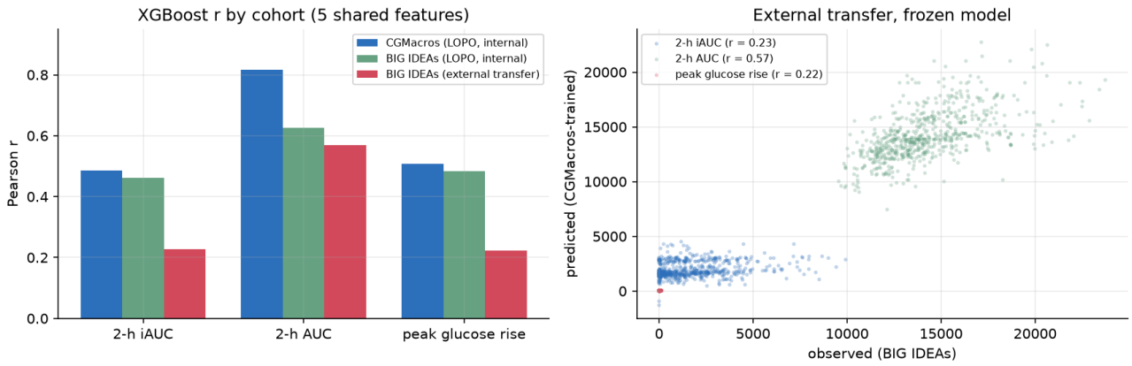
Figure 5 — External validation. Left: XGBoost Pearson r by cohort and target under the five shared features; the red bars are the frozen-model transfer. Right: predicted versus observed for the transferred model — the AUC cloud follows the diagonal loosely, while iAUC and peak rise are nearly flat.
