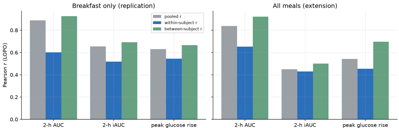
Pooled skill vs. within- and between-subject skill (XGBoost)
