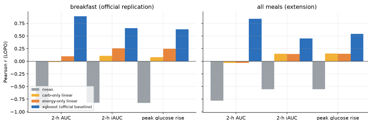
Figure 2 — Model comparison. Out-of-fold Pearson r by model, target and subset. XGBoost dominates everywhere; the linear baselines are close to zero, and the mean predictor is negative by construction. The sign is worth explaining: under LOPO the "mean" model predicts the mean of the other 44 subjects, so for a high-responding person that mean is pulled down by that person's own exclusion. The leave-one-out mean is therefore anti-correlated with the held-out subject, which is why this no-skill reference lands below zero (and below 0.5 ROC-AUC) instead of at zero. It is a reference point, not a model that has learned anything.
