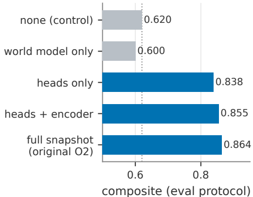
(a) the ceiling is policy-head memory
