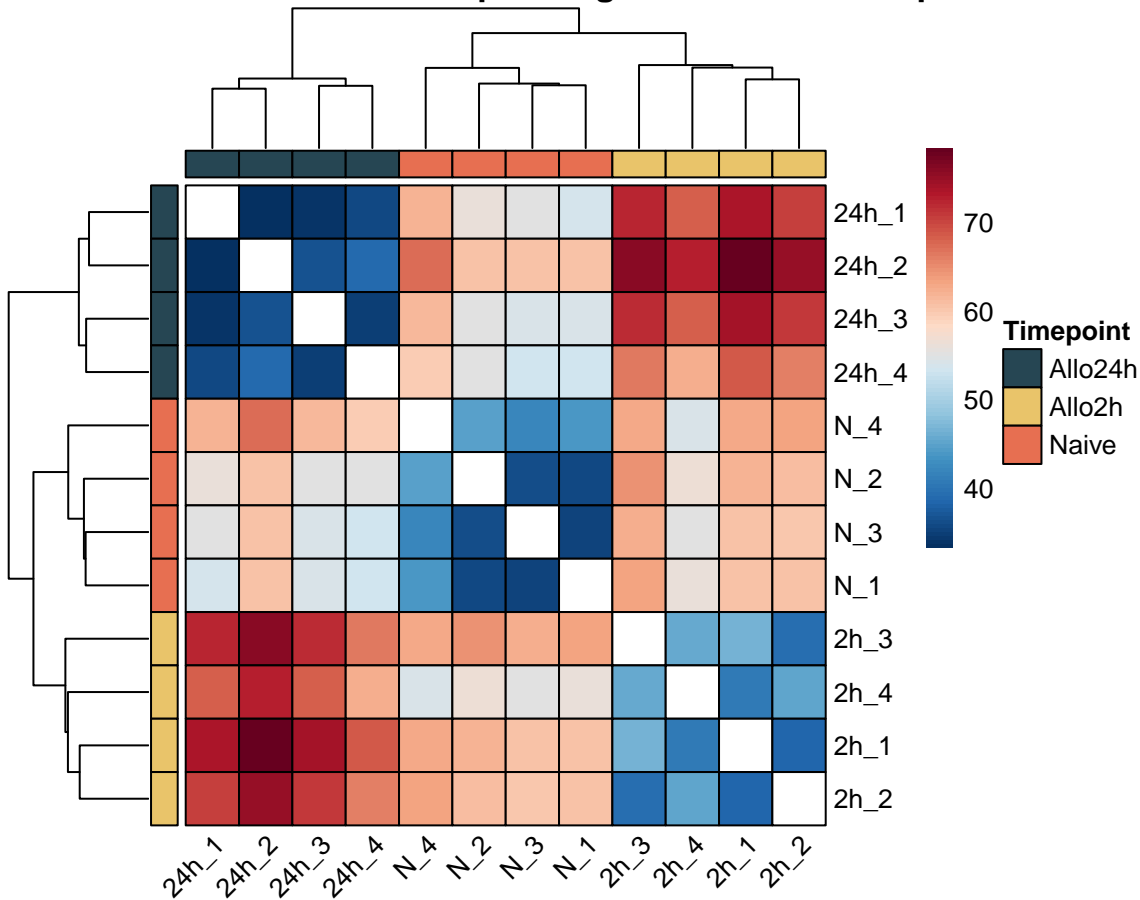
Euclidean Distance Heatmap of log-transformed samples
