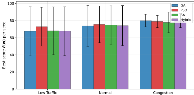
Variability of best score across seeds (mean \pm std, n=3 )
