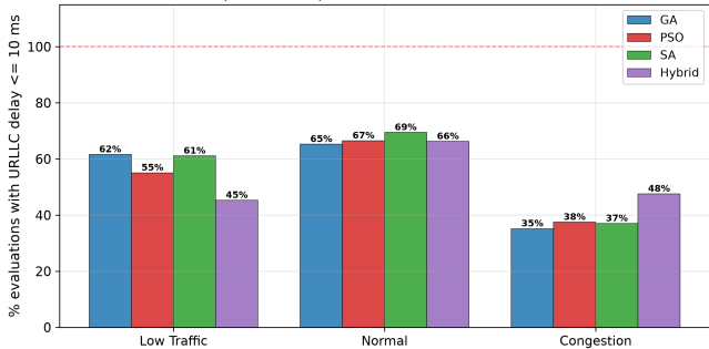
URLLC SLA compliance rate per meta-heuristic (URLLC-active evaluations)
