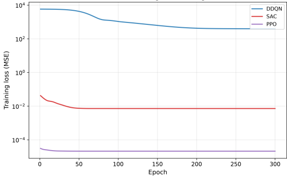
Offline DRL training: loss convergence
