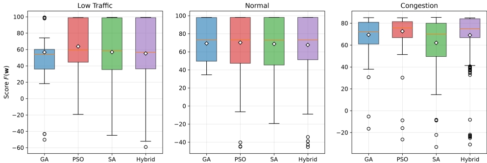
Score distribution per meta-heuristic and scenario (3 seeds, diamond = mean)
