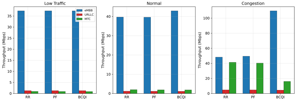
Throughput per slice and scenario - pure schedulers (mean of 3 seeds)
