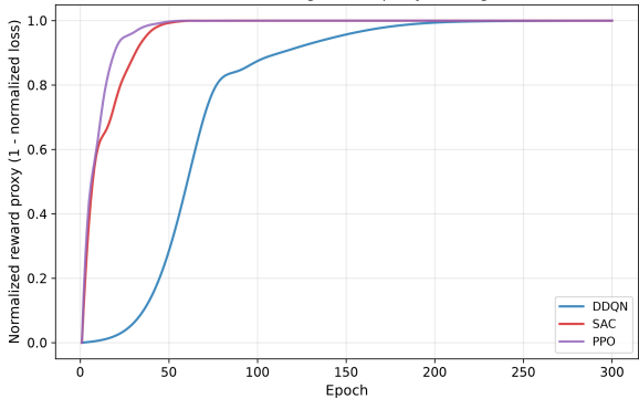
Offline DRL training: reward proxy convergence
