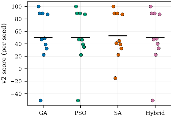
low_traffic — seed dispersion
