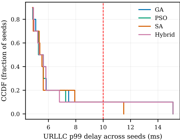
low_traffic — tail spread
