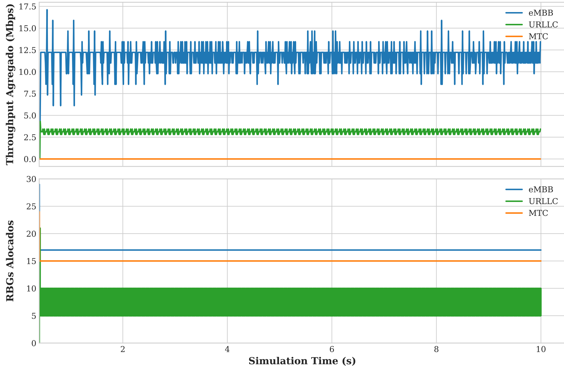
Network Performance with Static Allocation (No DRL) Scenario: Last Executed — Aggregated Throughput per Slice
