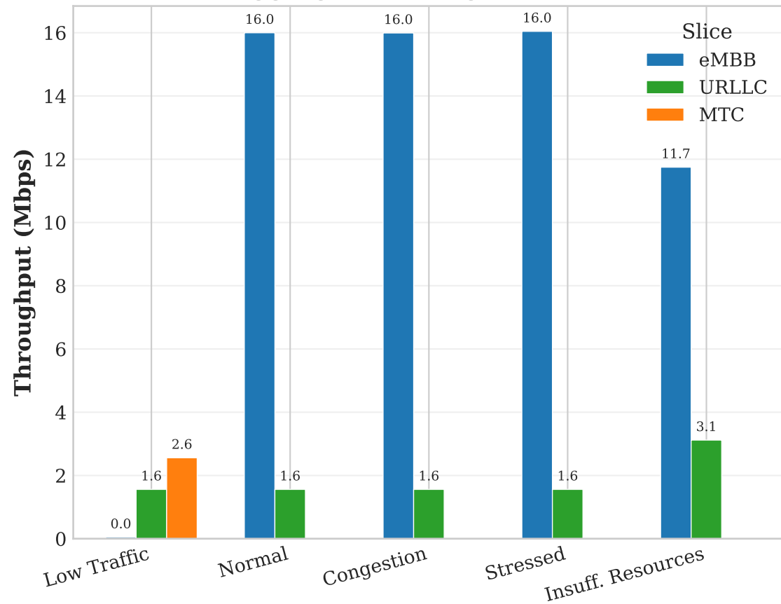
(a) Aggregate Throughput per Slice
