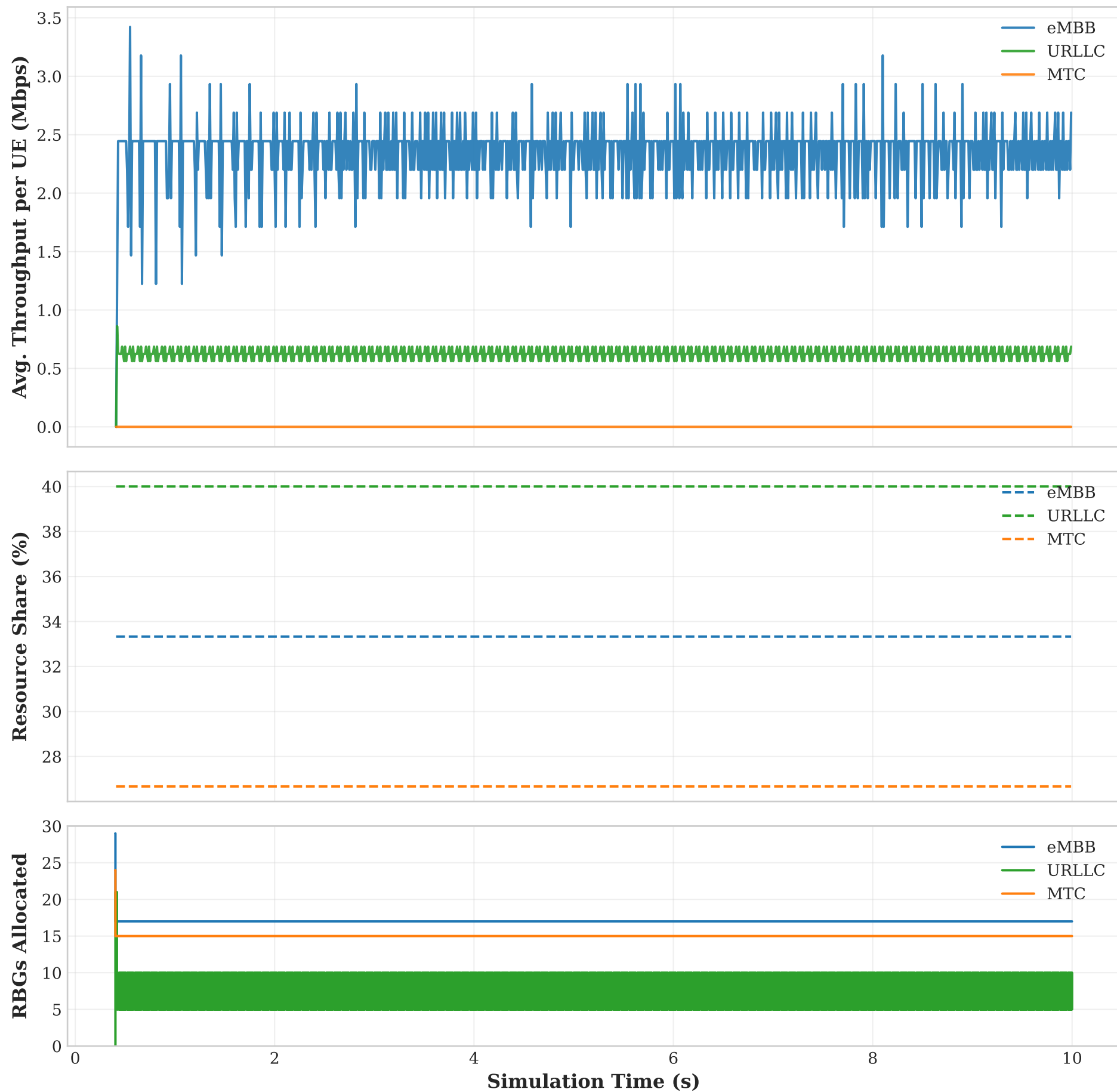
Static Slice-Aware Baseline — Per-UE Metrics Over Time
