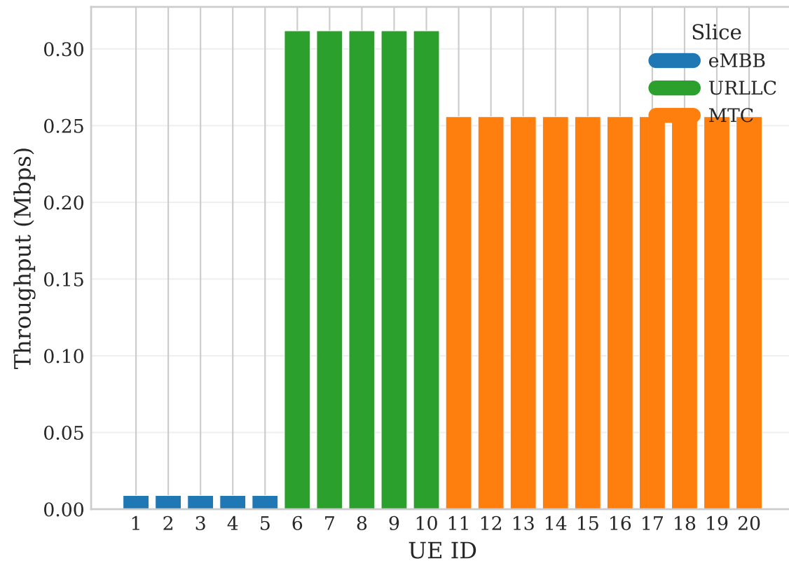
(a) Low Traffic — All Slices Served
