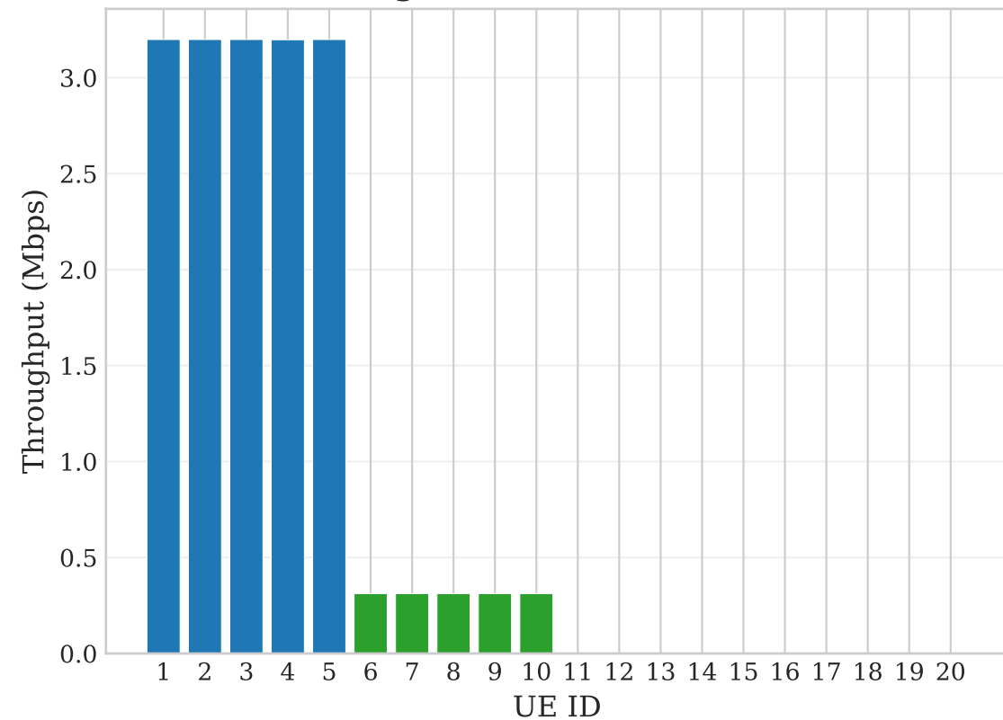
(b) Congestion — MTC Starvation
