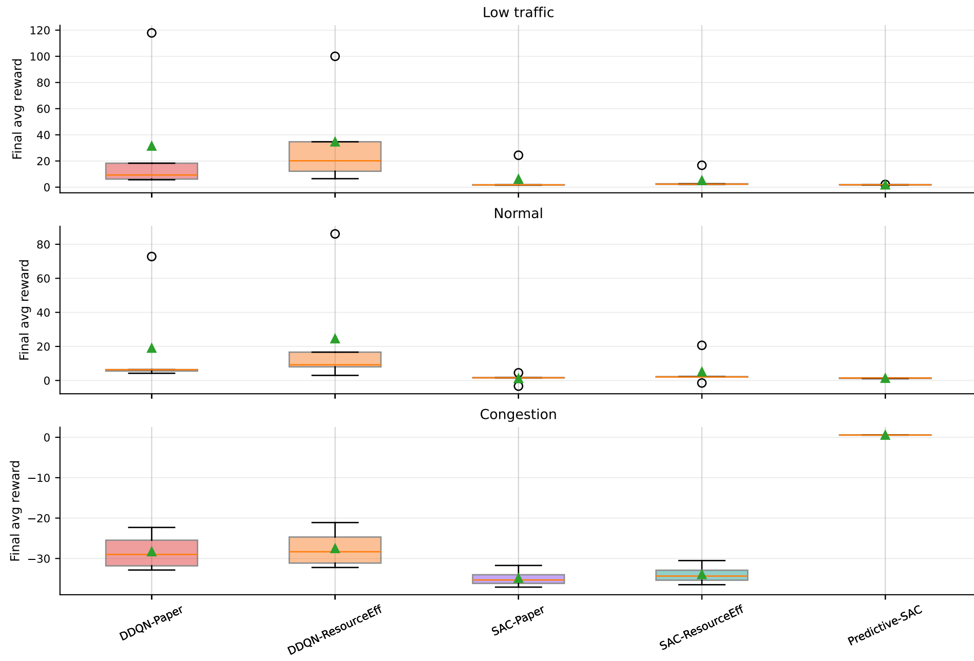
Training reward final_avg_100 by method
