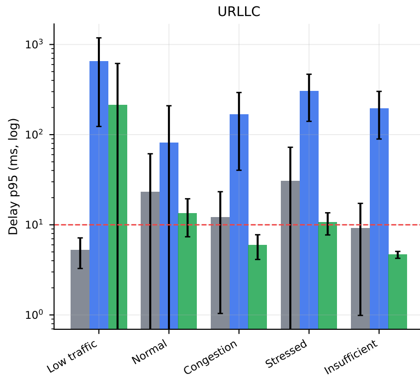
Baseline latency vs 3GPP-inspired service expectations
