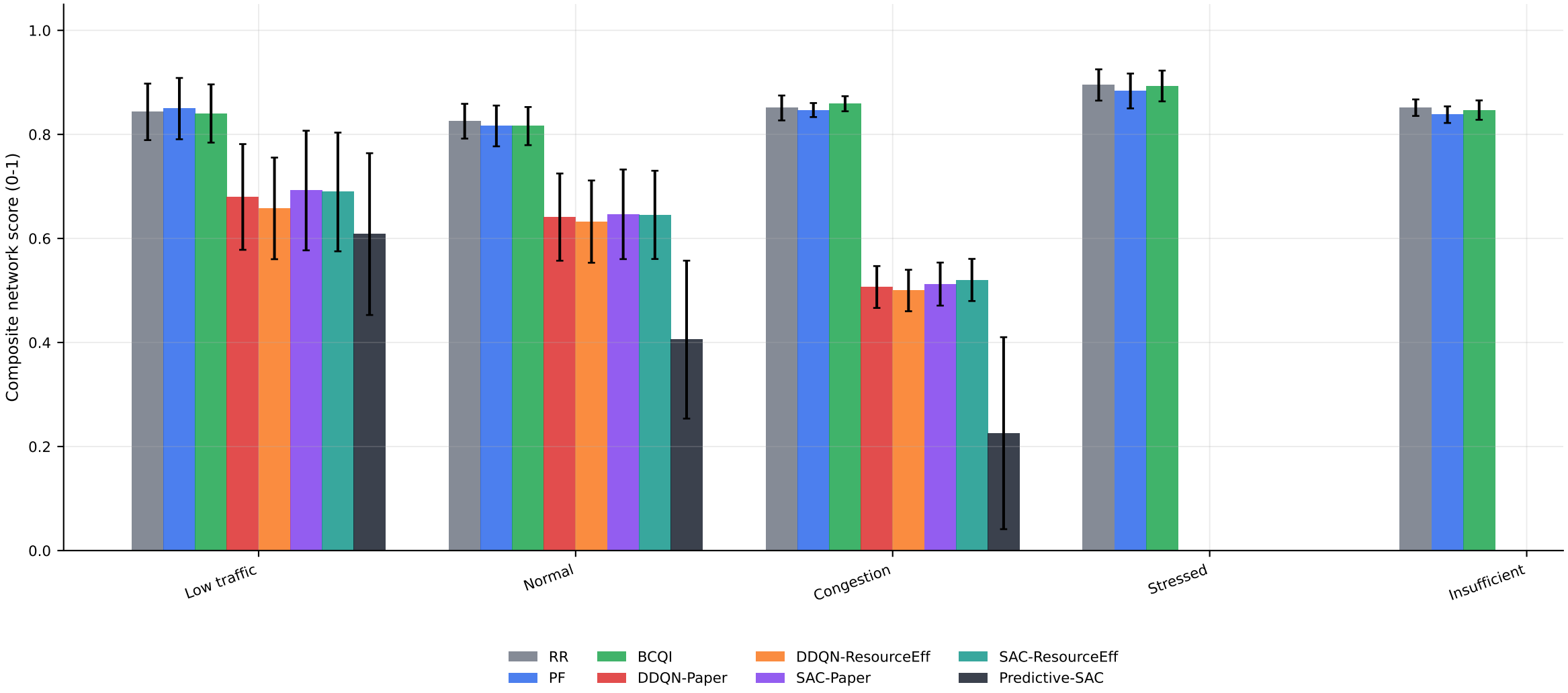
QoS/SLA composite score from common available metrics
