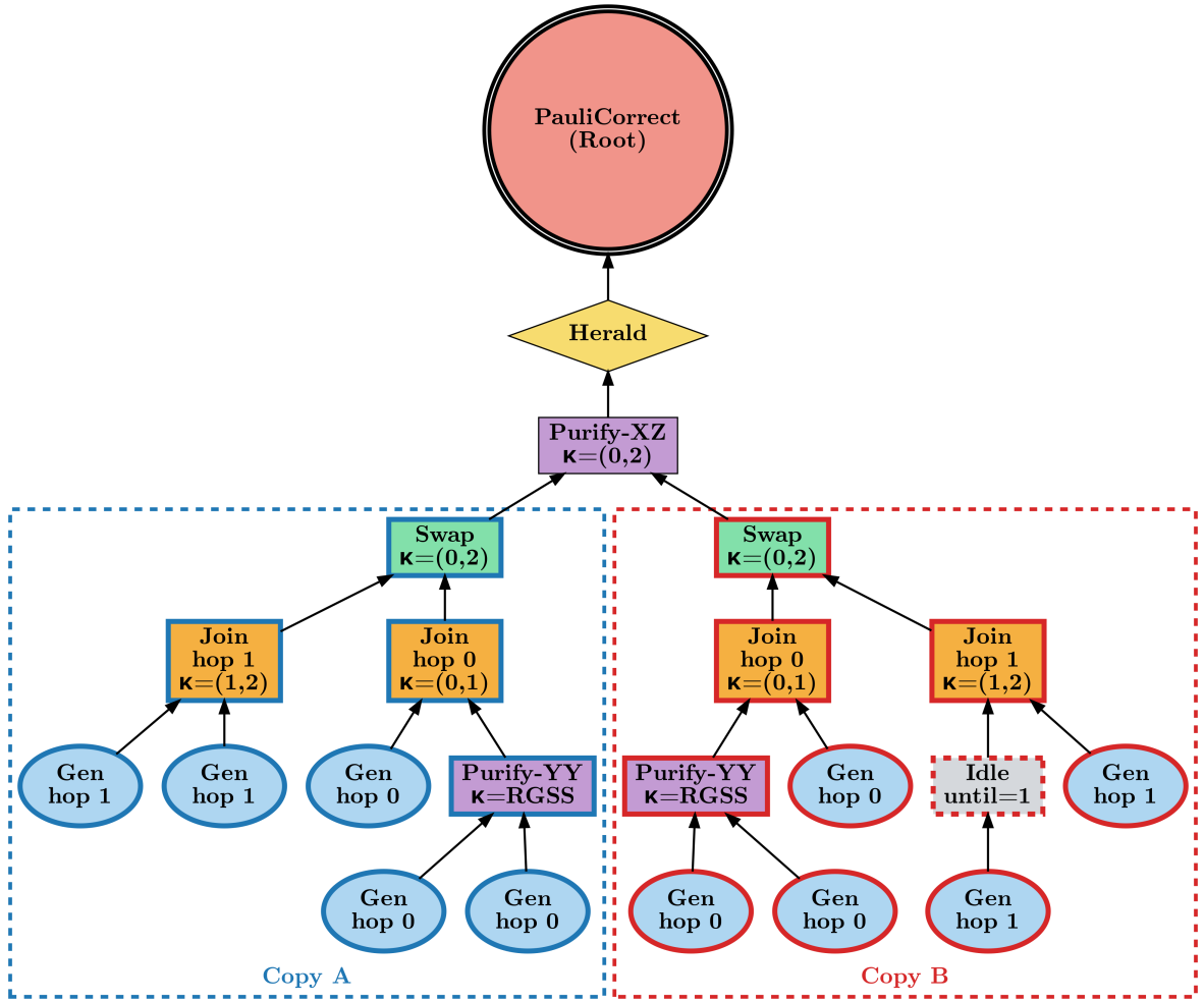
Figure 4.1: N = 2 example schedule \Sigma illustrating all seven node types ( C(\Sigma) = 10 GenNode leaves). [color in blue: Copy A ] (left subtree): hop 0 applies PurifyNode-YY at \kappa = \text{RGSS} before the outer-photon JoinNode ; hop 1 is raw. [color in red: Copy B ] (right subtree): identical except the right-side hop-1 GenNode is wrapped in an IdleNode (grey, dashed) modelling a synchronisation wait before the JoinNode . The two copies are first combined into \kappa = (0, 2) by a SwapNode , then purified together by PurifyNode-XZ . The single HeraldNode placed after (not before) PurifyNode-XZ makes this an optimistic schedule (Section 4.3). PauliCorrectNode is the root at \kappa = (0, 2) . Edges run bottom-to-top.
