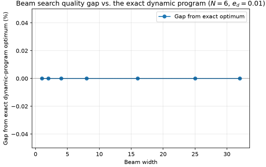
Figure A.2: Beam search’s rate gap from the exact dynamic-program optimum vs. beam width, at N = 6 , e_d = 0.01 .
