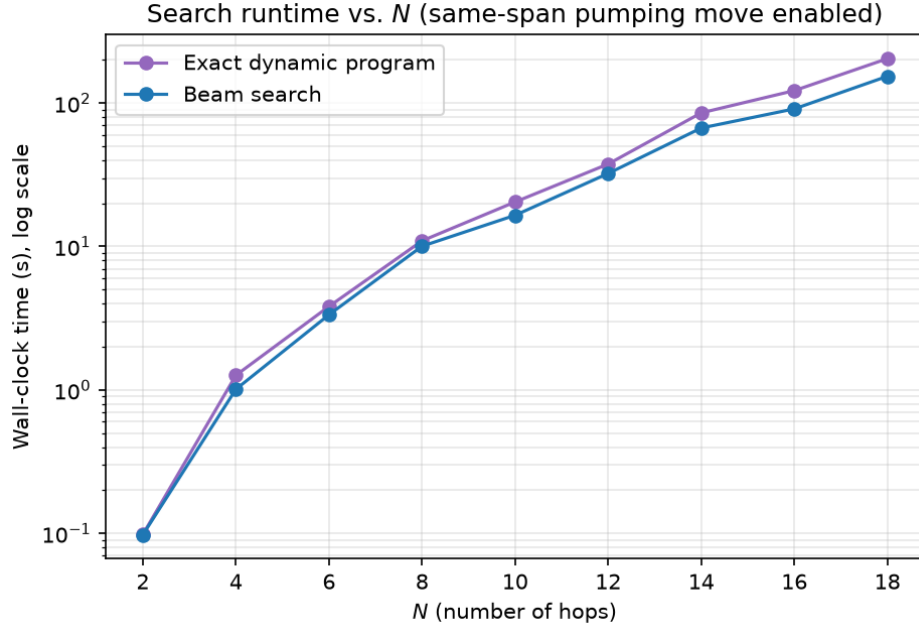
Figure A.3: Search wall-clock time vs. N for the exact dynamic program and the beam search, same-span pumping move enabled throughout.
