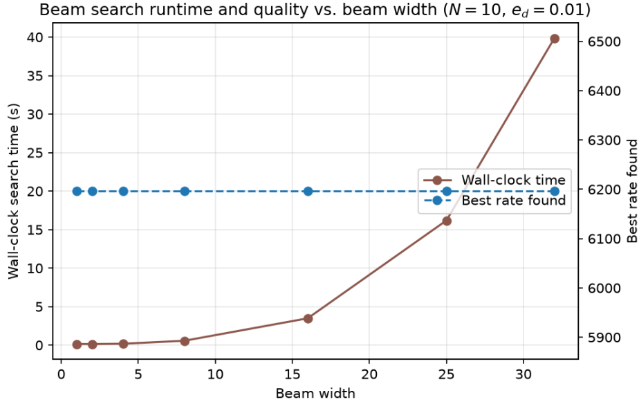
Figure A.1: Beam search wall-clock time and best rate found vs. beam width, at N = 10 , e_d = 0.01 .
