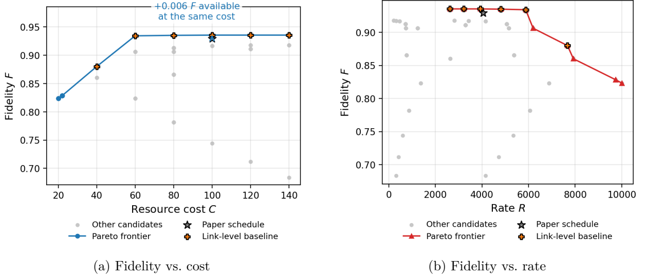
Figure 6.3: Pareto frontiers at N = 10 , e_d = 0.01 , E_{\max} = 150 , over candidates evaluated under a permissive objective ( F_{\min} = 0 ). Grey points are dominated; connected points form the non-dominated frontier, with the paper schedule and uniform link-level baseline marked for reference.
