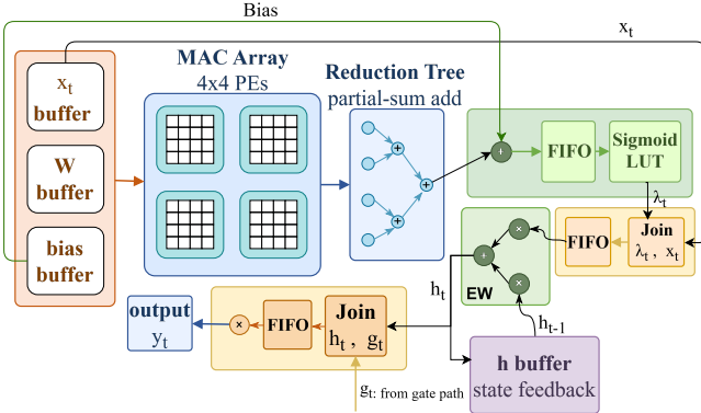
Fig. 4. Slim-Mamba state-update datapath.
