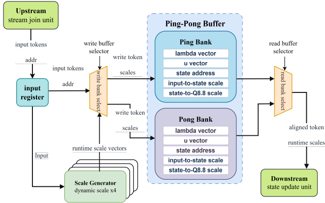
Fig. 7. Ping-pong scale-buffer organization for aligning token, state address, update coefficient, and runtime scale streams.
