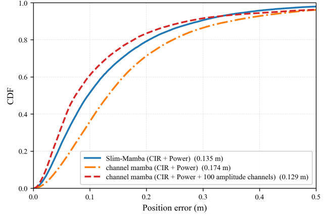
Fig. 8. Cumulative distribution of localization error for Slim-Mamba and two CMamba reference runs under matched-input and augmented-input settings.
