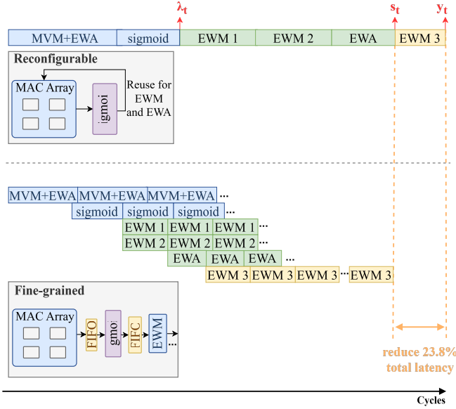
Fig. 3. Comparison between coarse-grained and fine-grained scheduling.
