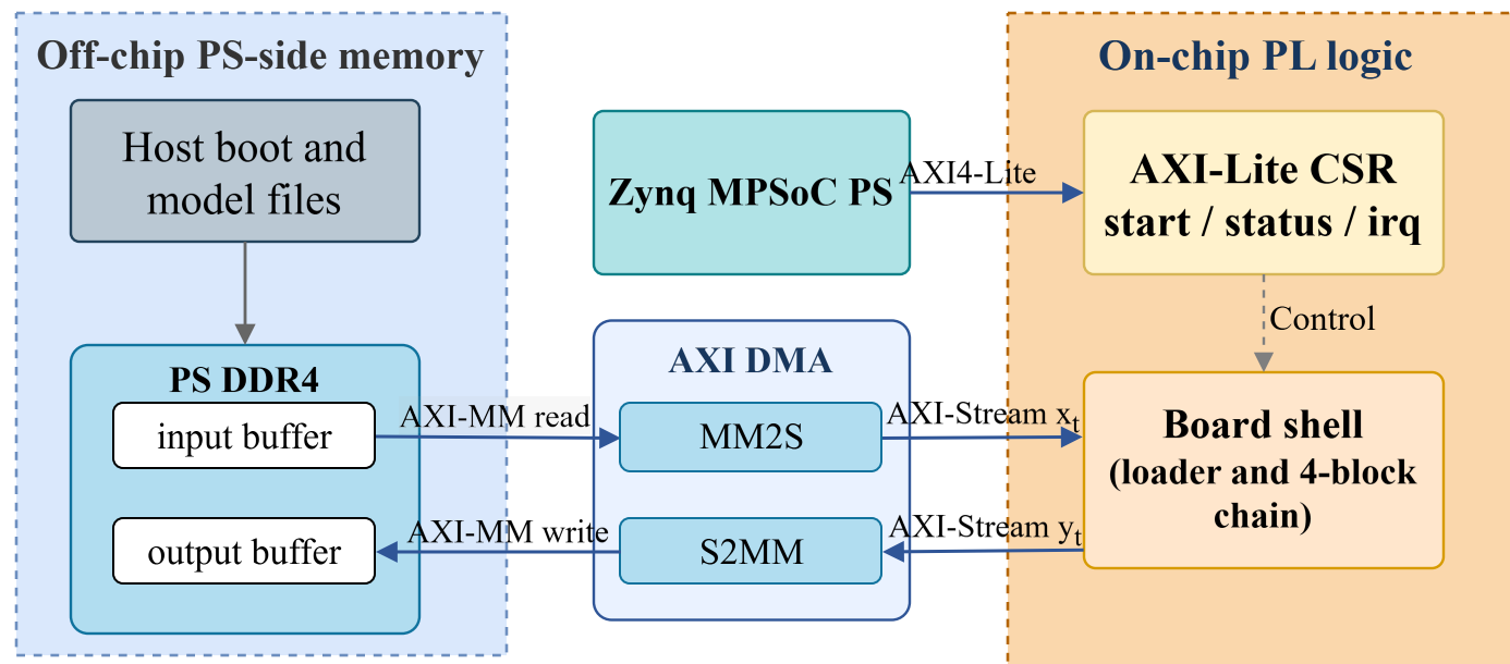
(a) Board-level memory and AXI interfaces
