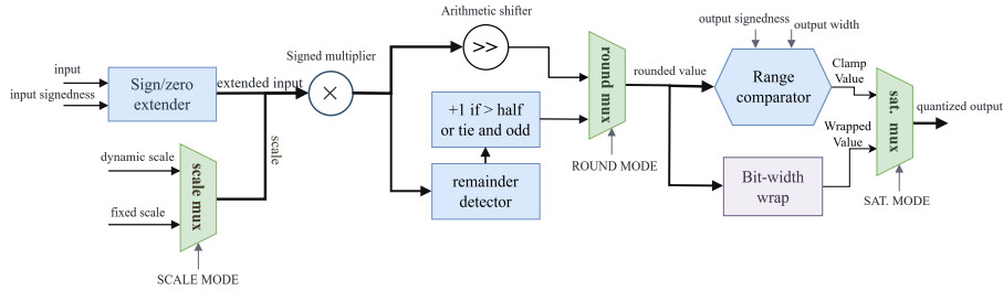
Figure 4.10: Configurable fixed-point quantization engine for one vector lane.
