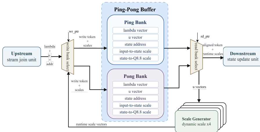
Figure 4.11: Ping-pong buffer alignment for runtime dynamic scales in the selective-scan path.
