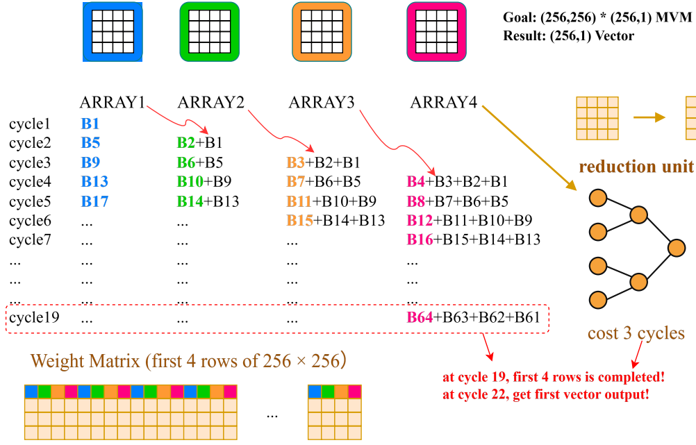
Fig. 6. 4 × 4 × 4 arrays organization.
