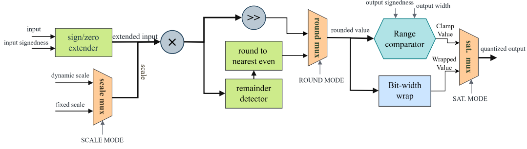
Fig. 3. Configurable fixed-point requantization engine reused across projection, state-update, and residual paths.
