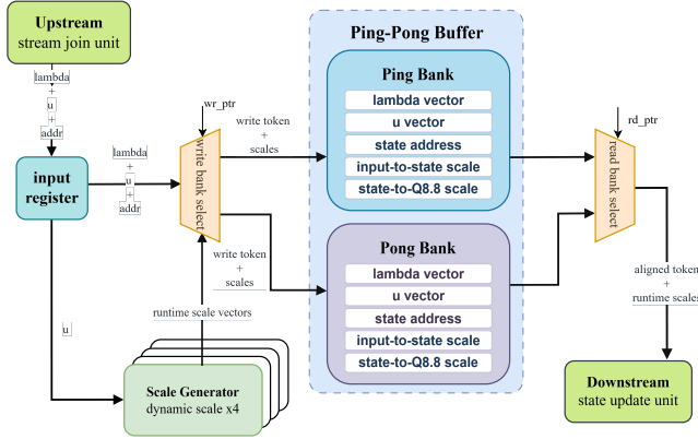
Fig. 4. Ping-pong scale-buffer organization for aligning token, state address, update coefficient, and runtime scale streams.
