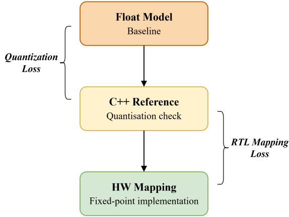
Fig. 1. The quantization tools: from floating-point evaluation to bit-true fixed-point modelling and RTL mapping.
