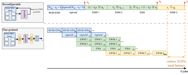
Fig. 7. Comparison between coarse-grained and fine-grained scheduling.
