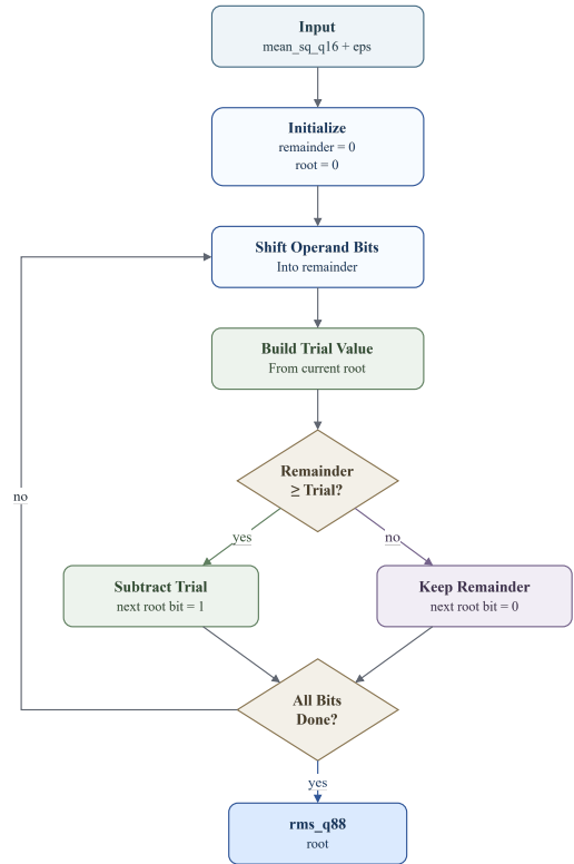
Fig. 8. RMSNorm approximation flow: a trial-quotient digit-recurrence procedure.
