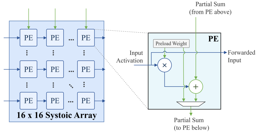
Figure 4.2: An example of Systolic Array.
