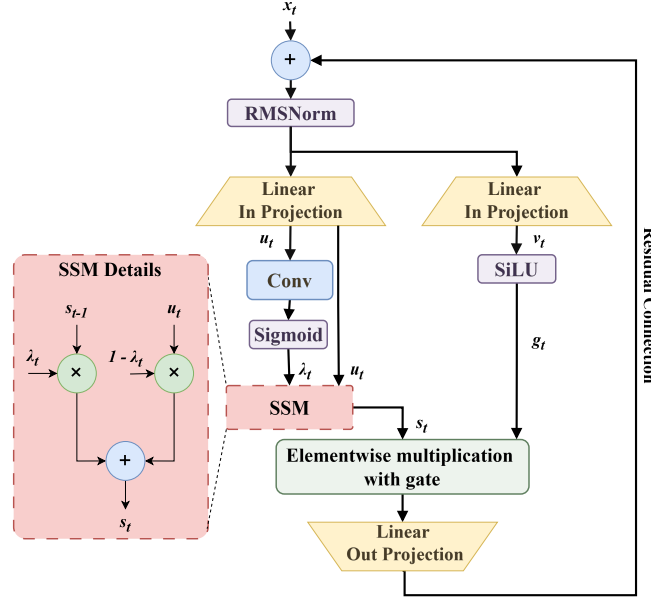
Figure 3.2: Simplified datapath of the Slim Mamba block.
