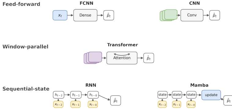
Figure 3.1: Comparison of common localization backbones in terms of how temporal context is represented and how data dependencies are introduced during inference.
