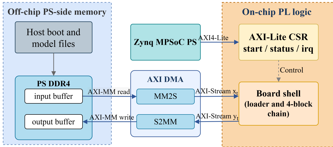
(a) Board-level memory and AXI interfaces
