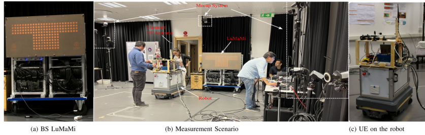
Figure 1.1: Massive MIMO indoor localization measurement setup with moving user equipment, adapted from [4].
