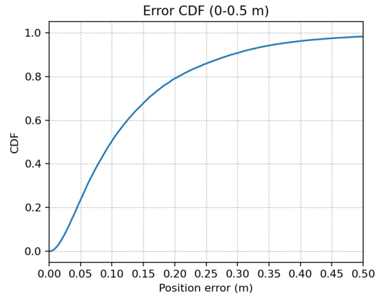
Figure 4.1: CDF of localization error for the evaluated software models.
