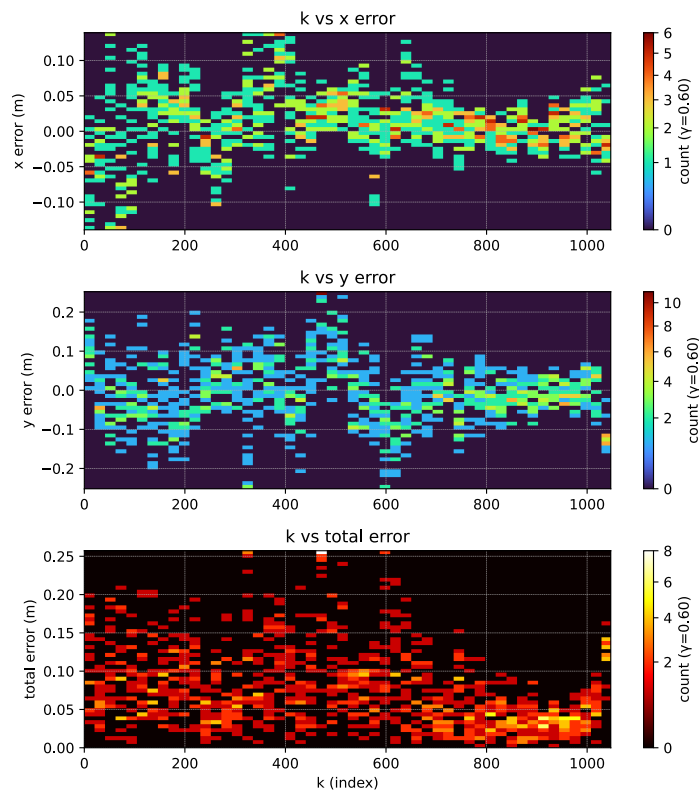
Figure 4.2: Error heatmap for grid 102.
