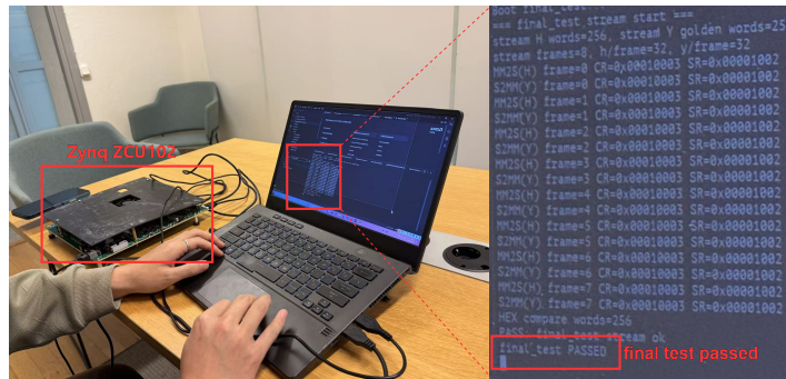
Figure 4.3: FPGA on-board validation flow.
