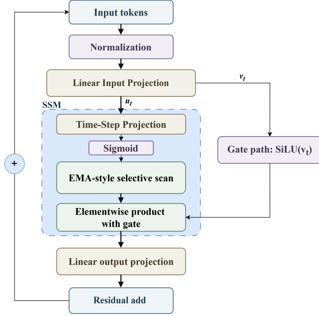
Figure 3.1: Simplified datapath of the Slim Mamba block.
