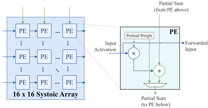
Figure 4.2: An example of Systolic Array.
