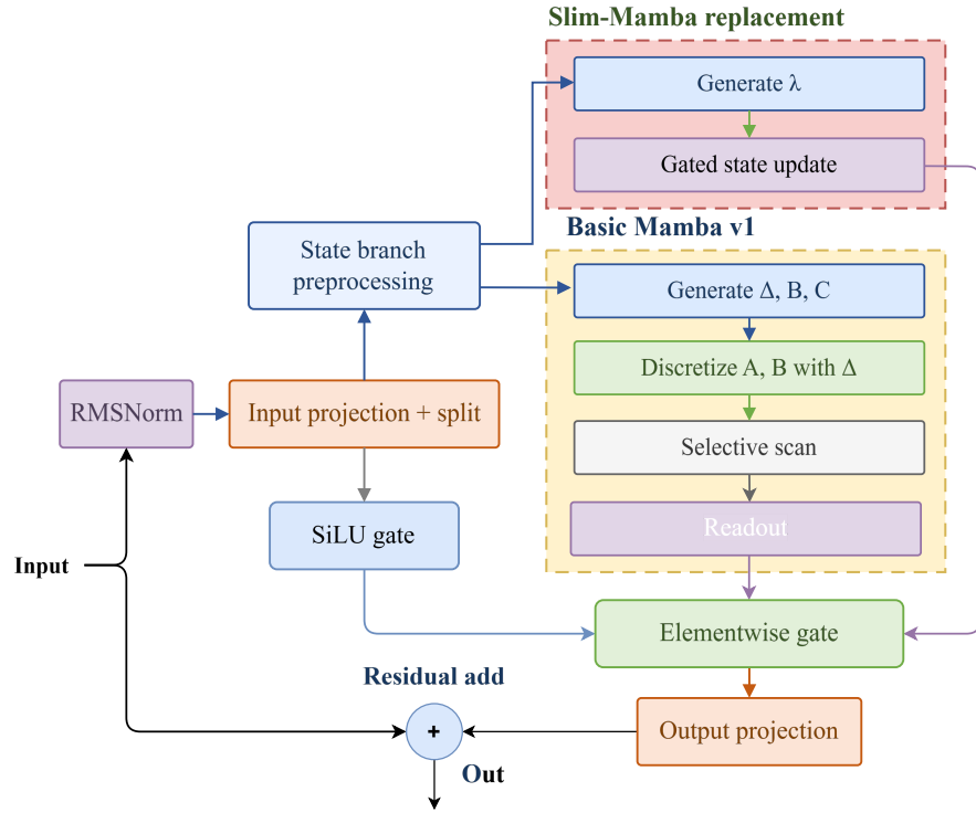
Figure 3.2: Original Mamba block and its Slim-Mamba replacement.
