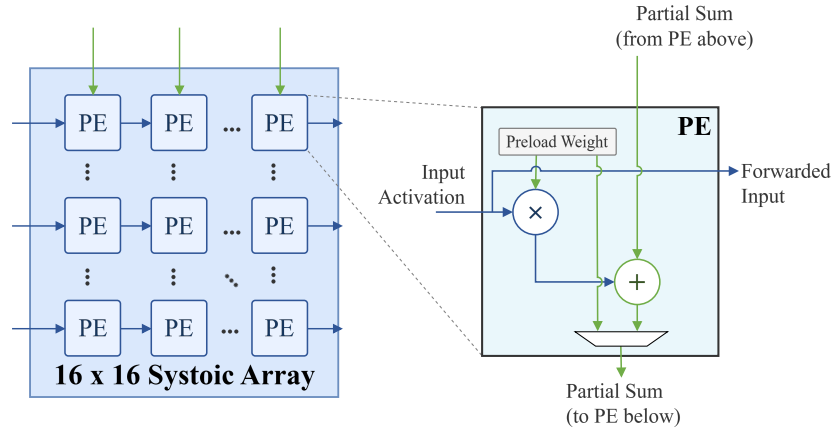
Figure 4.2: Example of a systolic array.
