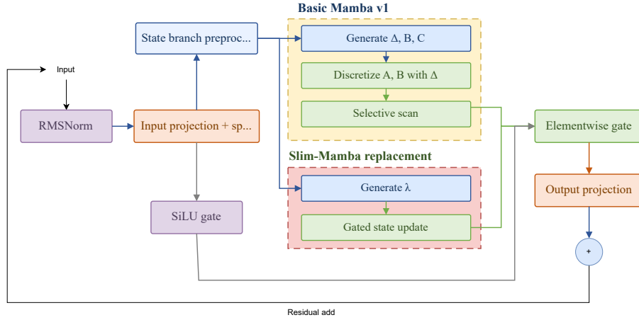
Figure 3.2: Original Mamba block and its Slim-Mamba replacement.
