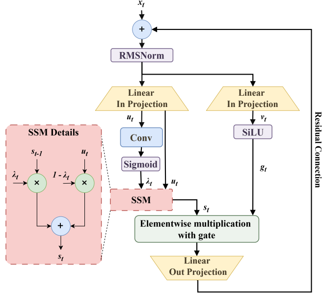
Figure 3.3: Simplified datapath of a Slim-Mamba block.
